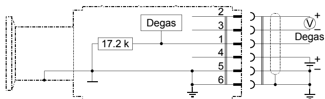
Figure 1: Electrical connection
