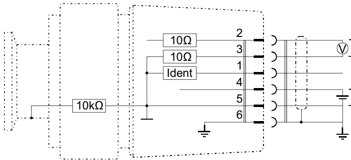
Fig. 4: Connection diagram
