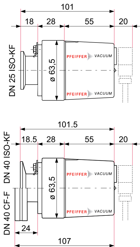
Fig. 17: Dimensions
