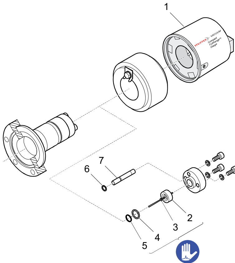
Fig. 15: Spare parts
